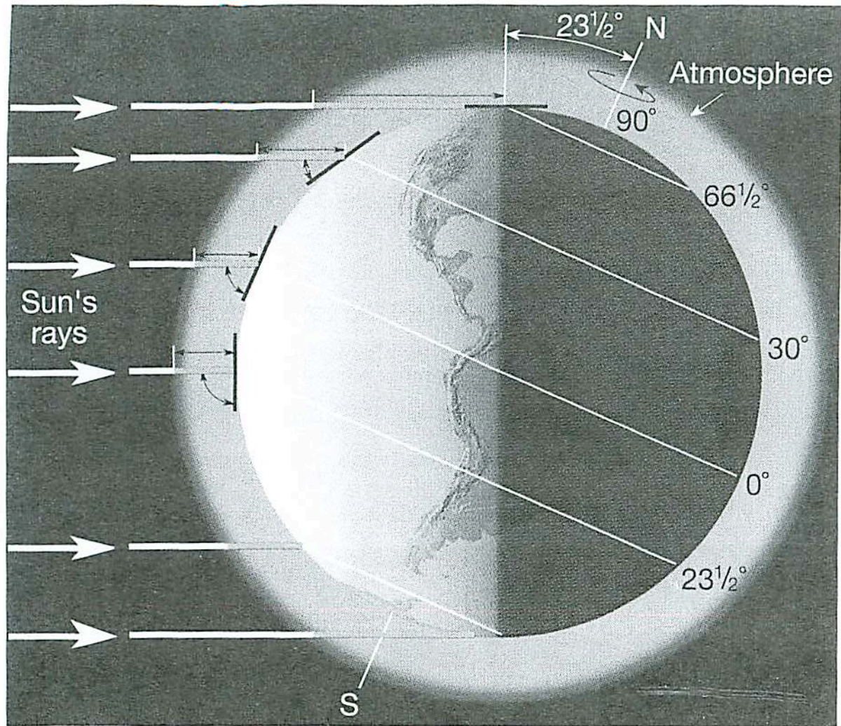
FIGURE 2-2 2-1 Rays striking Earth at a low angle (toward the poles) must traverse more of the atmosphere than rays striking at a high angle (around the equator) and thus are subject to greater depletion by reflection and absorption.
